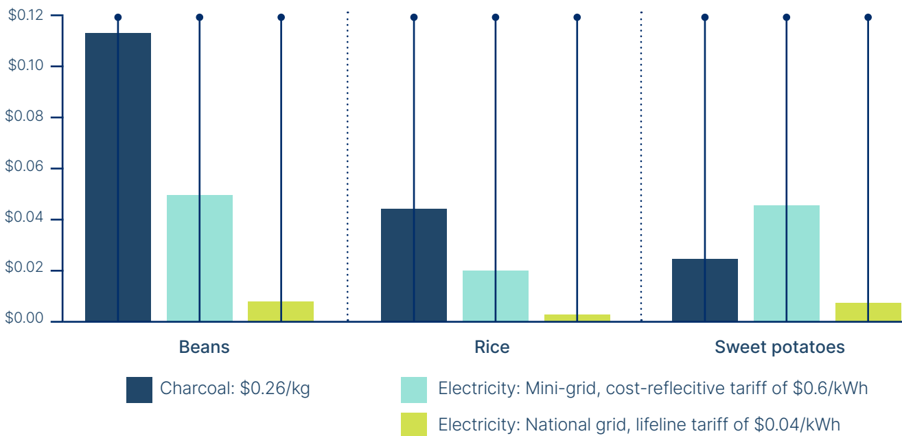
Graph 1: A study in Tanzania found that cooking with electricity was cost competitive when a cost-reflective, mini-grid tariff is applied and cheaper when on the national grid compared to charcoal. From “Costs of cooking with different fuels a case study from mini-grids in Tanzania” by Inston, R. & Scott, N., 2022, MECS. 6
