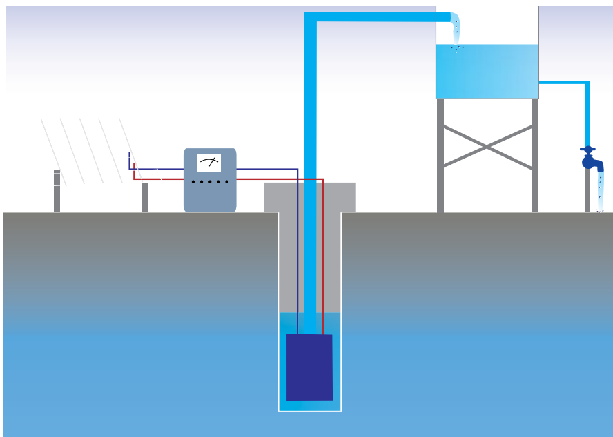
Figure 2: Drinking water system using a submersible pump. Source: RENAC.
